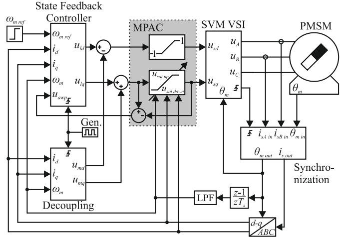
Fig. 3. Schematic block diagram of PMSM drive system with SFC and MPAC algorithm.
