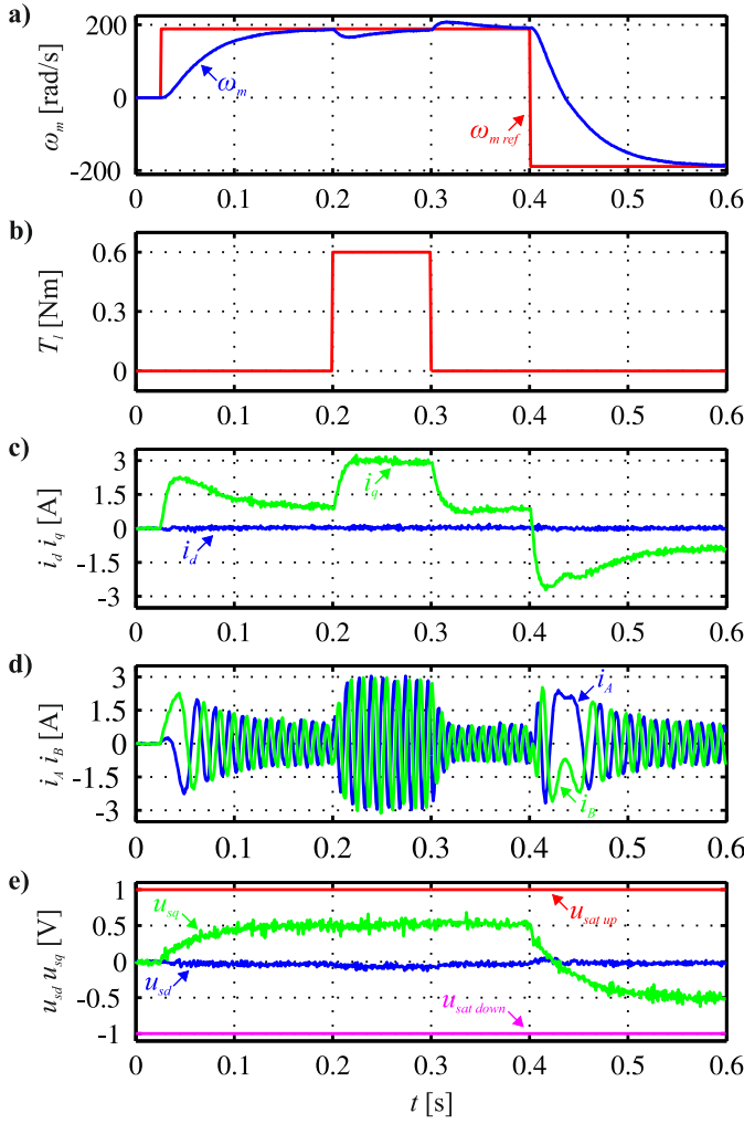
Fig. 8. The experimental response of the PMSM drive with non-constrained SFC to step changes of the reference angular velocity and load torque: a) speed reference and feedback, b) load torque reference, c) q -axis and d -axis currents, d) phase currents, e) d - q control voltages and q -axis constraints.
