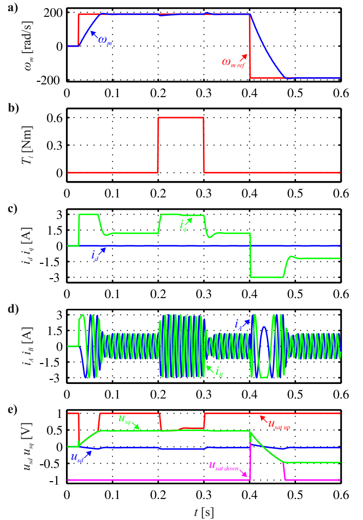
Fig. 4. The simulation response of the PMSM drive with SFC and MPAC to step changes of the reference angular velocity and load torque: a) speed reference and feedback, b) load torque reference, c) q -axis and d -axis currents, d) phase currents, e) d - q control voltages and q -axis constraints.
