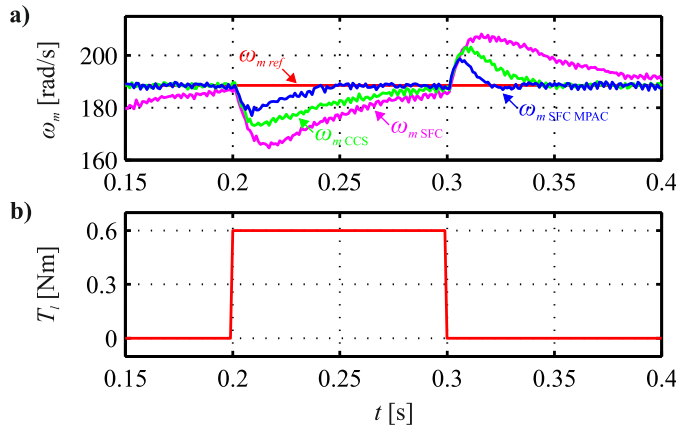
Fig. 10. The experimental response of the PMSM drive with non-constrained SFC, SFC with MPAC and CCS to step changes load torque: a) speed reference and feedback, b) load torque reference.
