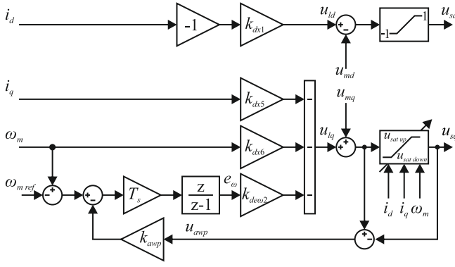
Fig. 1. Block diagram of the designed state feedback controller with MPAC and anti-windup.
