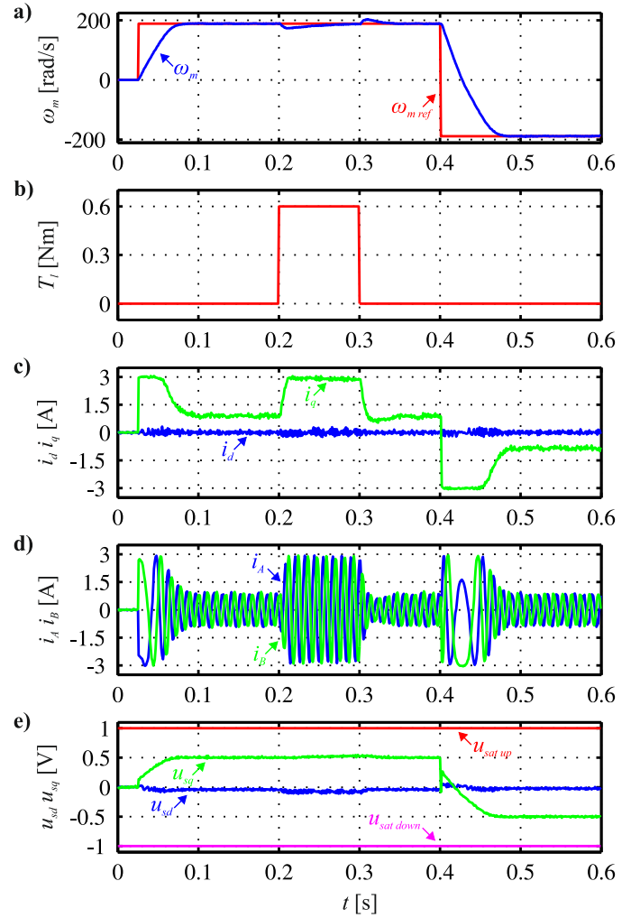
Fig. 9. The experimental response of the PMSM drive with CCS to step changes of the reference angular velocity and load torque: a) speed reference and feedback, b) load torque reference, c) q -axis and d -axis currents, d) phase currents, e) d - q control voltages and q -axis constraints.
