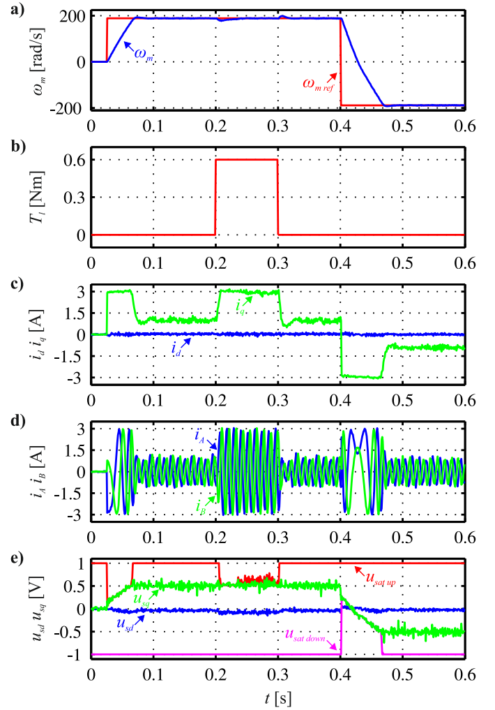
Fig. 7. The experimental response of the PMSM drive with SFC and MPAC to step changes of the reference angular velocity and load torque: a) speed reference and feedback, b) load torque reference, c) q -axis and d -axis currents, d) phase currents, e) d - q control voltages and q -axis constraints.
